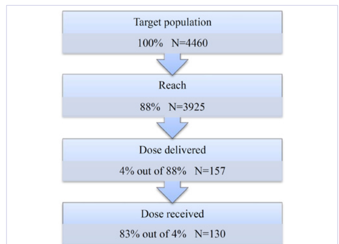
Figure 1: Quantitative results
